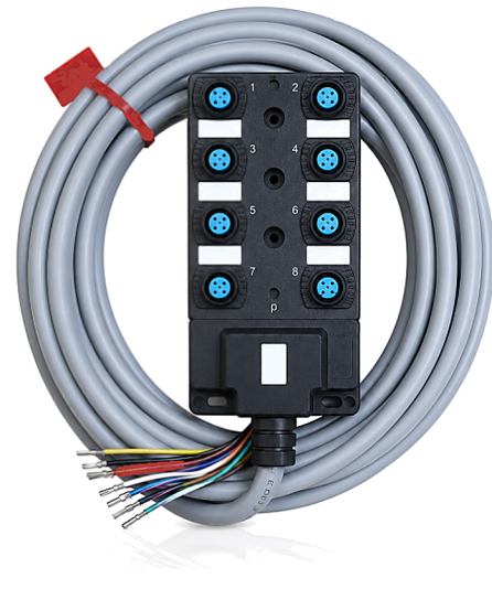
VXT-JB-M12-08D-10M shown · 8-port body with moulded 10 m master cable
