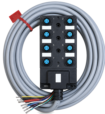
VXT-JB-M12-08D-05M shown · 8-port body with moulded 5 m master cable
